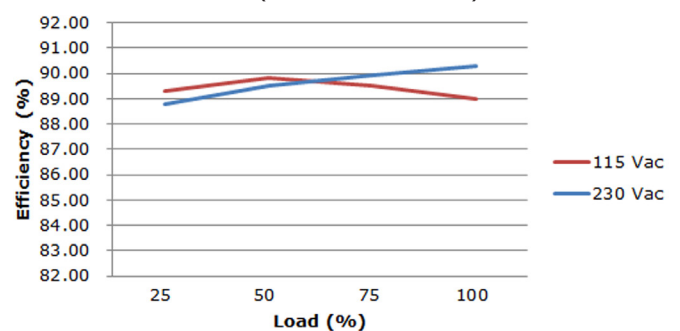
VOF-85B-24 Efficiency vs. Output Load (Natural Convection)
