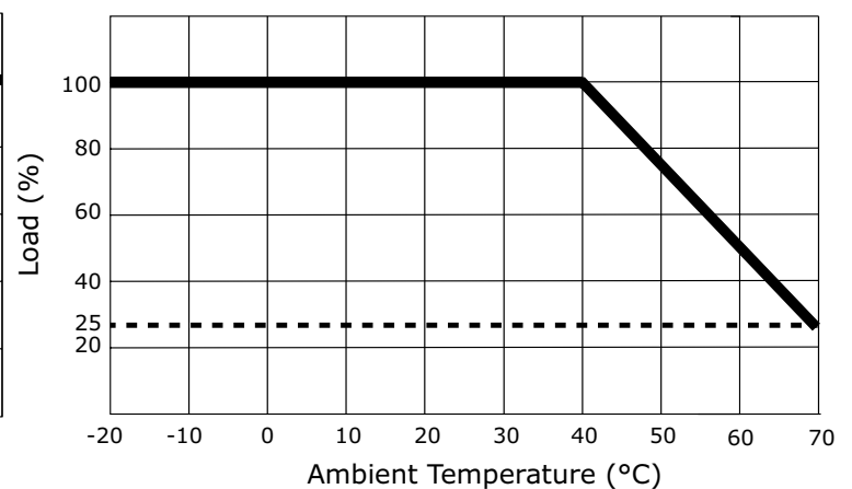
Output Load vs. Ambient Temperature
