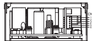
cross sectional view A Scale 1:1
