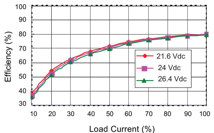
PCSA1-S24-S12-S Efficiency Curve (Efficiency vs. Line Voltage and Load Current)
