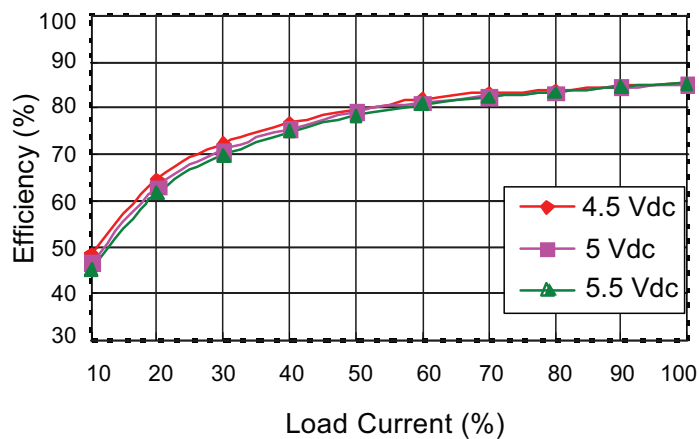
PCN2-S5-D5-S Efficiency Curve (Efficiency vs. Line Voltage and Load Current)
