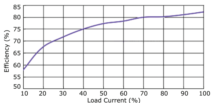
AE15-UW-S24 Efficiency Curve Efficiency vs. Load Current
