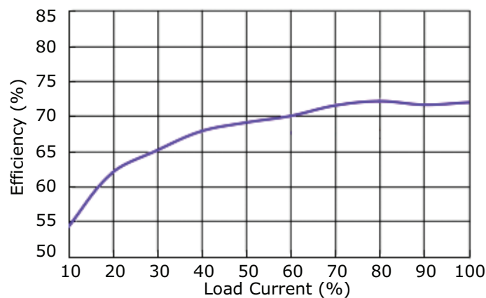
Efficiency Curve Efficiency vs. Load Current
