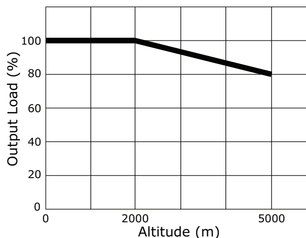
Load vs. Altitude Derating Curve
