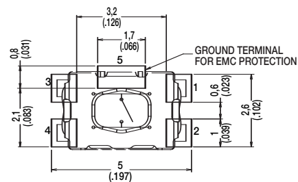
PAD LAYOUT
