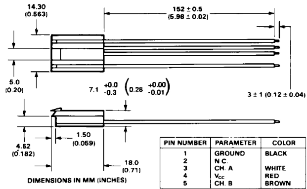
Figure 6. HEDS-8902 Connector.
