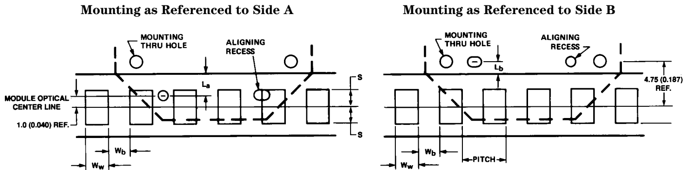
Figure 4. Codelistrip Design
