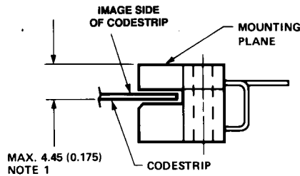
Mounting Plane Side A
