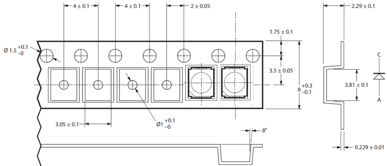
Figure 11. Tape dimensions.
