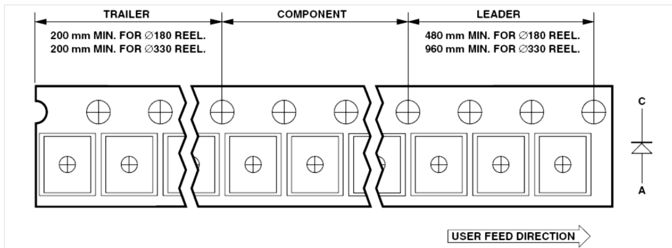
Figure 10. Tape leader and trailer dimensions.
