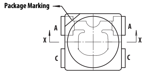
Figure 11b. Component Axis for Radiation Pattern
