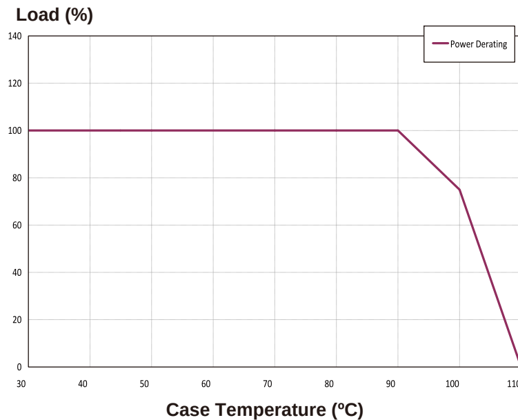
Power Derating vs Case Temperature
