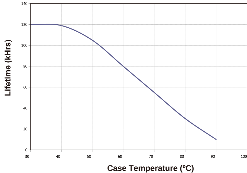
Lifetime vs Case Temperature
