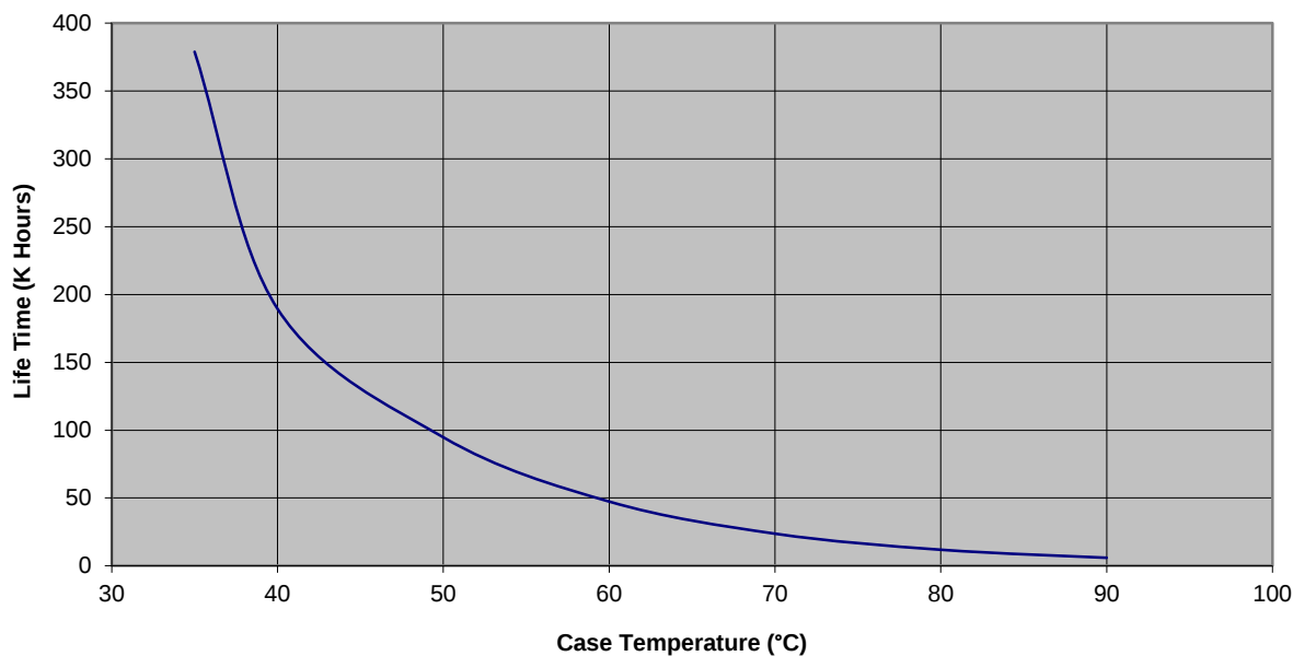
Life Time vs Case Temperature 42V @ 485VAC
