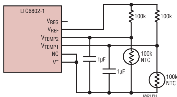
Figure 14. Driving Thermistors Directly from V_{\text{REF}}
