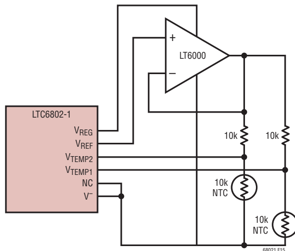
Figure 15. Buffering V_{\text{REF}} for Higher-Current Sensors
