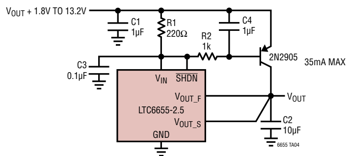
Boosted Output Current
