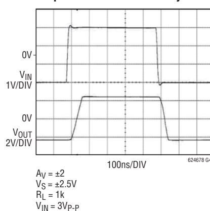
Output Overdriven Recovery
