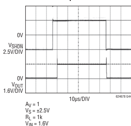
\overline{SHDN} Pin Response Time
