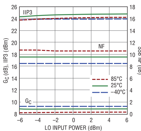
2600MHz Conversion Gain, IIP3 and NF vs LO Power
