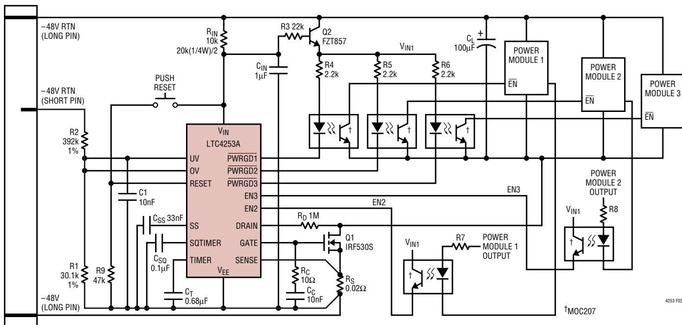
Figure 3. -48V/2.5A Application for the LTC4253A
