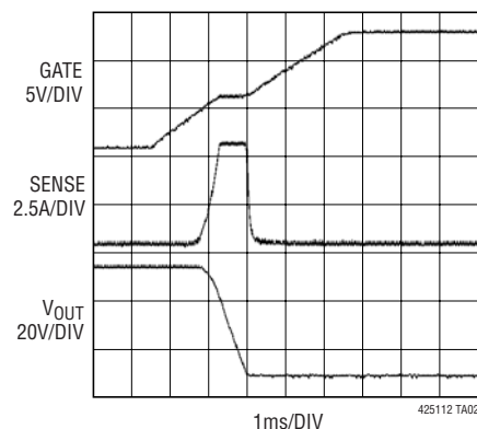
Start-Up Behavior
