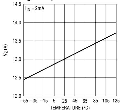
V_Z vs Temperature
