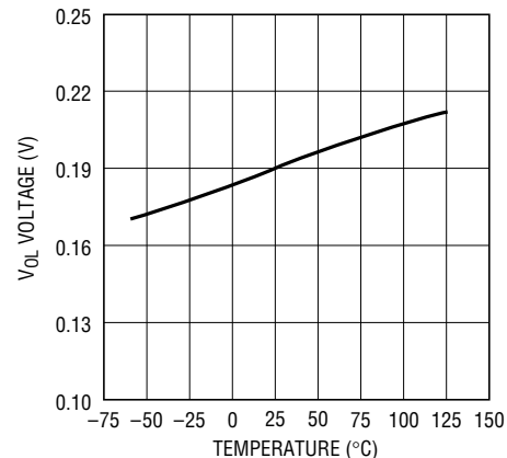
V_{OL} (RESET \overline{n} , FAULT) vs Temperature
