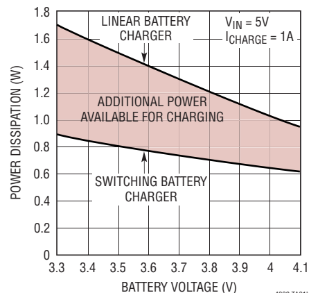
Reduced Power Dissipation vs Linear Battery Charger
