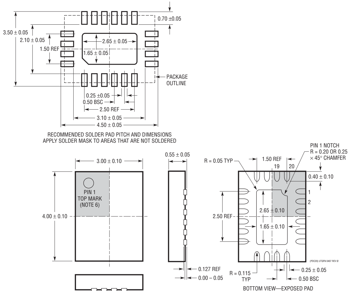
PDC Package 20-Lead Plastic UTQFN (3mm × 4mm) (Reference LTC DWG # 05-08-1752 Rev 0)
