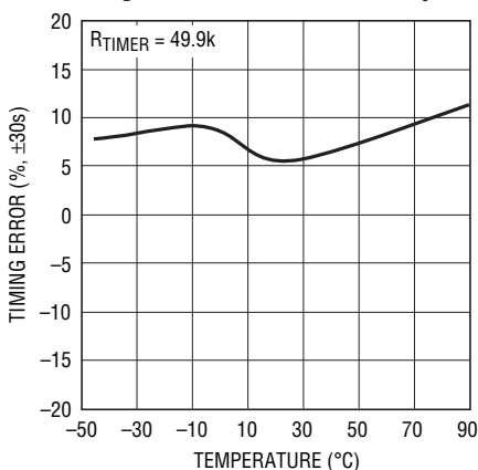
Programmable Timer Accuracy
