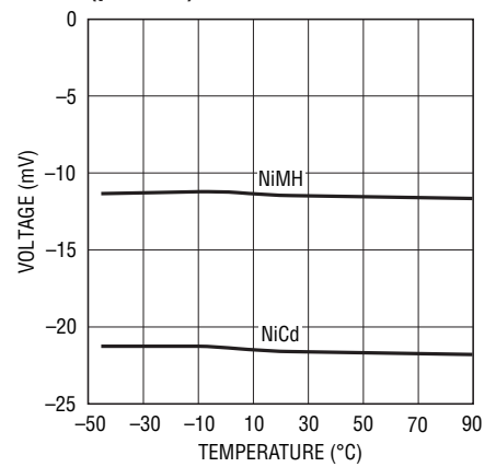
-\Delta V Termination Voltage (per Cell)
