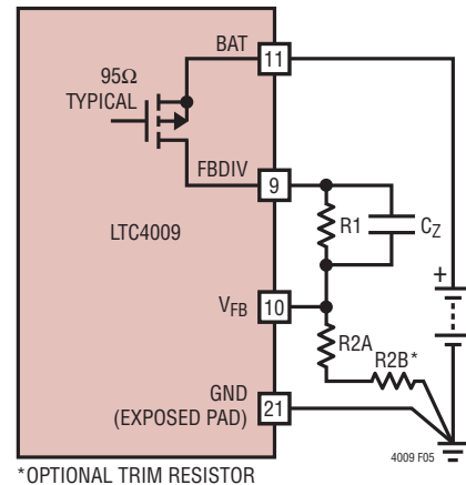
Figure 5. Programming LTC4009 Output Voltage
