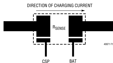
Figure 13. Kelvin Sensing of Charging Current
