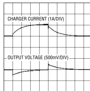
1A Load Step (Battery Present)
