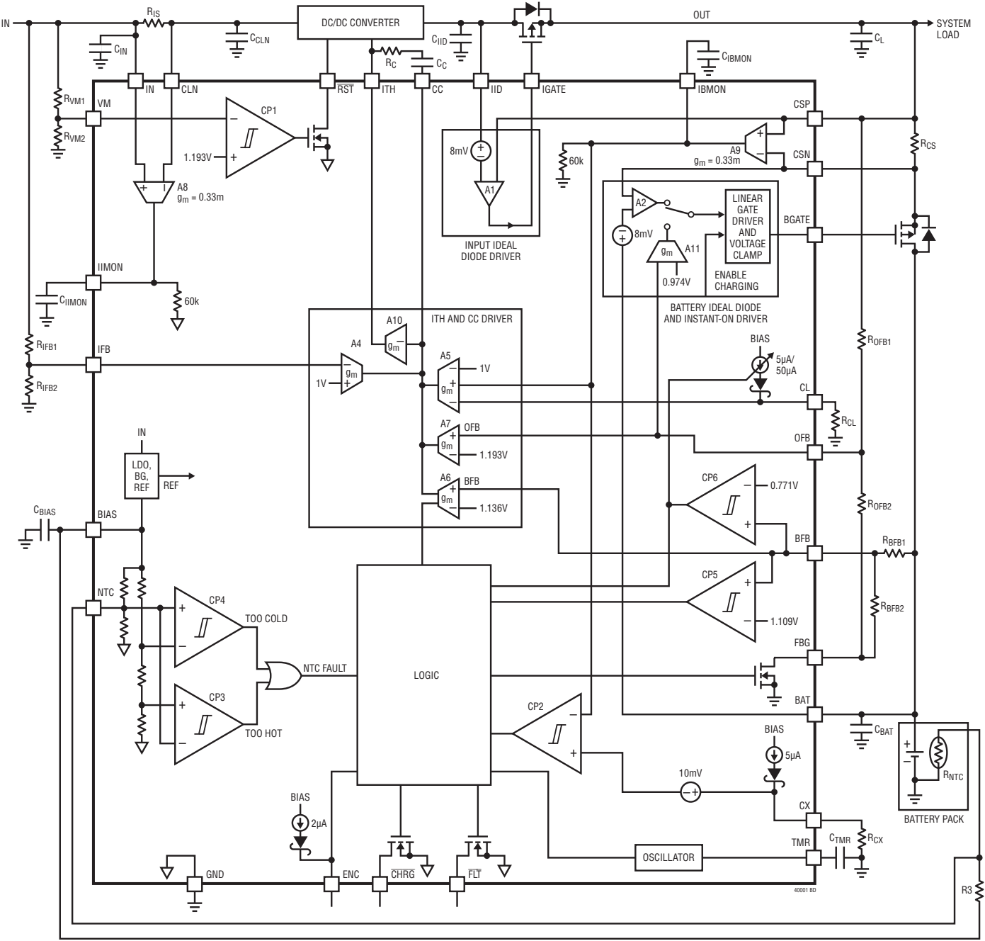
Figure 1. LTC4000-1 Functional Block Diagram
