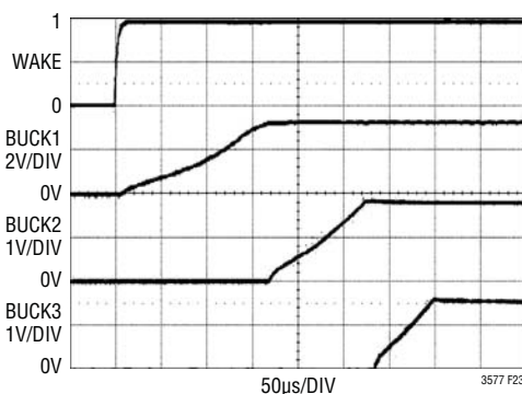
Figure 25. Power-Up Sequencing
