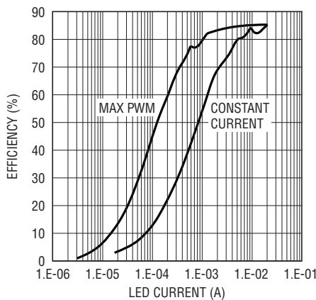
LED PWM vs Constant Current Efficiency
