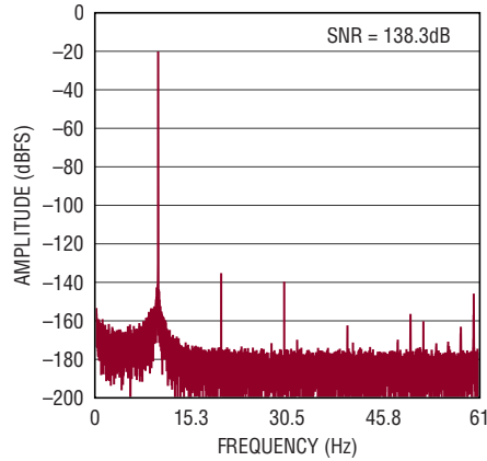
32k Point FFT f_{\text{SMPL}} = 2\text{Mpsps} , f_{\text{IN}} = 10\text{Hz} , N = 16384
