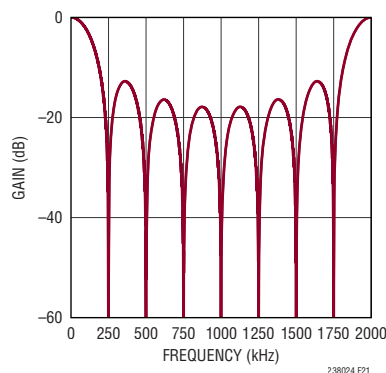
Figure 21. SINC 1 Filter with f_{\text{SMPL}} = 2\text{Mps} and N = 8
