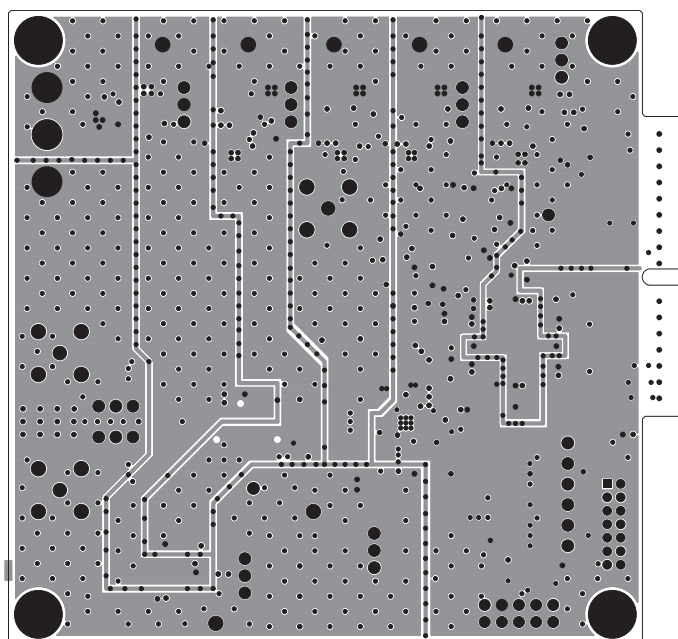
Layer 3 PWR Plane
