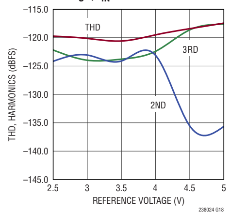
THD, Harmonics vs Reference Voltage, f_{\text{IN}} = 2\text{kHz}
