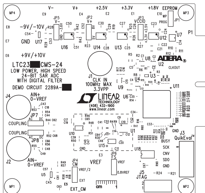
Top Silkscreen
