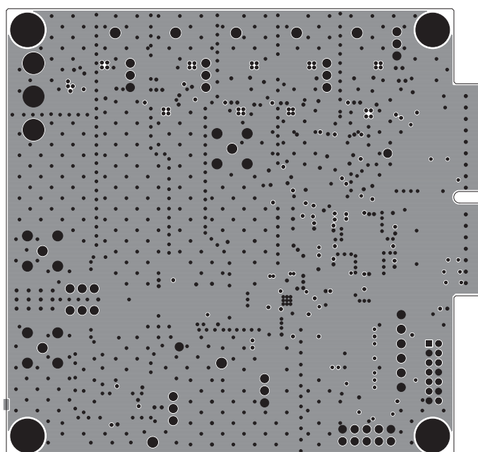
Layer 2 Ground Plane
