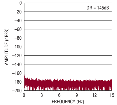
8k Point FFT f_{\text{SMPL}} = 2\text{Mpsps} , \text{IN}^+ = \text{IN}^- = V_{CM} , N = 65536
