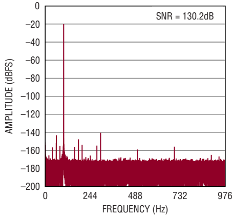
128k Point FFT f_{\text{SMPL}} = 2\text{Mpsps} , f_{\text{IN}} = 100\text{Hz} , N = 1024
