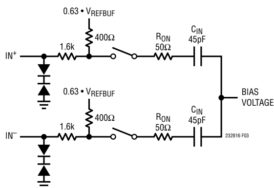
Figure 3. The Equivalent Circuit for the Differential Analog Input of the LTC2328-16
