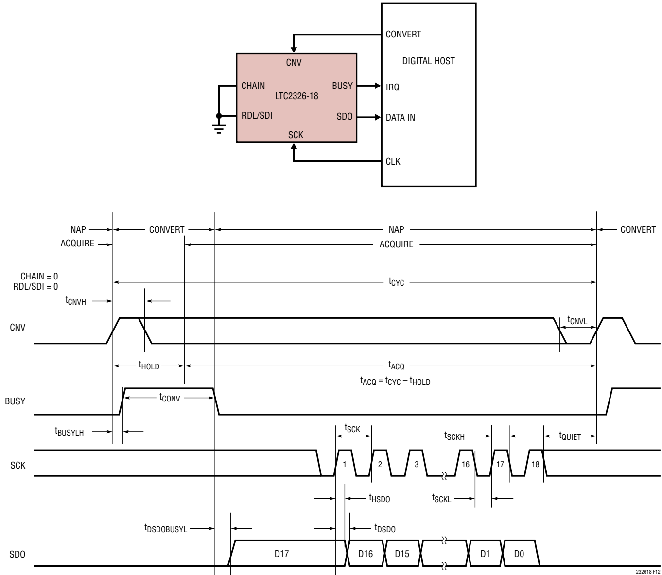
Figure 10. Using a Single LTC2326-18 in Normal Mode
