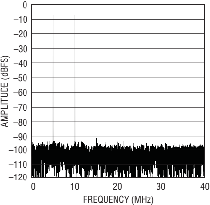
LTC2173-12: 8k Point 2-Tone FFT, f_{IN} = 70\text{MHz} , 75MHz, -1\text{dBFS} , 80Msps
