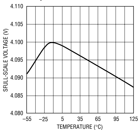
LTC1454 Full-Scale Voltage vs Temperature
