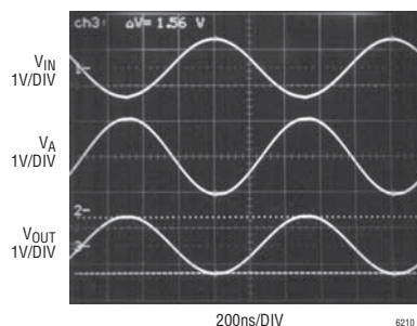
Figure 4. Response of Circuit at 1MHz
