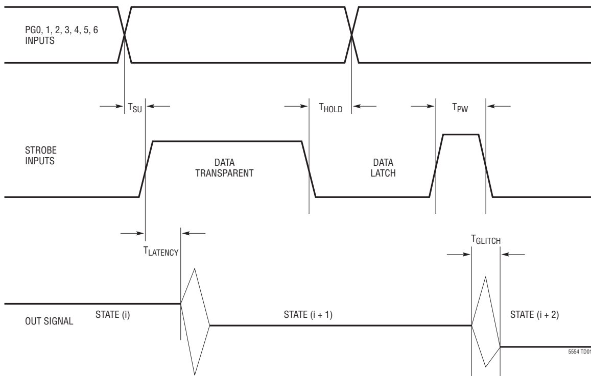
Timing Diagram
