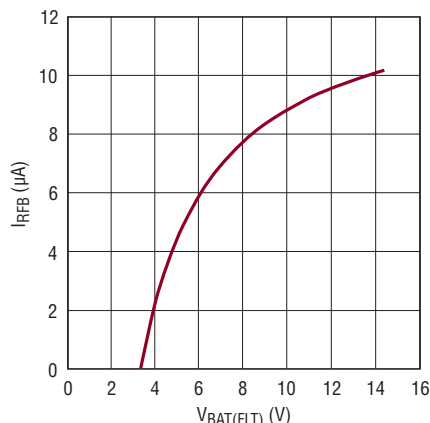
V_{\text{FLOAT}} Programming Resistor Current vs V_{\text{FLOAT}} for 2-Resistor Network
