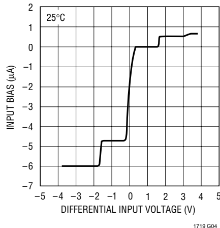
Input Current vs Differential Input Voltage
