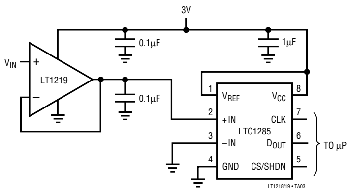
Buffer for 12-Bit A/D Converter
