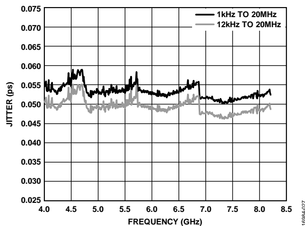
Figure 22. RMS Jitter, Fractional-N, f_{PFD} = 153.6 MHz, VCC\_VCO = 5 V
