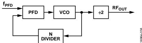
Figure 26. Loop Closed Before Output Divider
