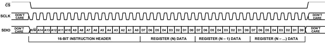
Figure 5. 3-Wire, MSB First, Descending Data, Streaming
