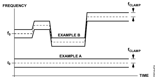
Figure 82. Example Frequency Clamp Plot
