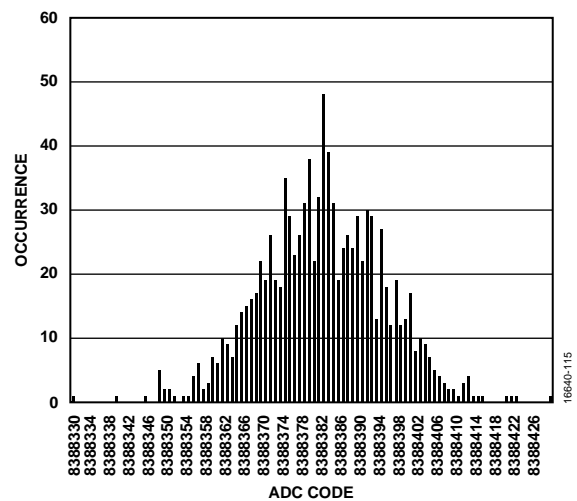
Figure 15. Histogram (Current Input, Output Data Rate = 31.25 SPS)
