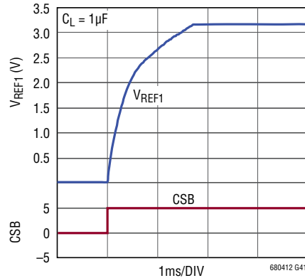
V_{REF1} Power-Up
