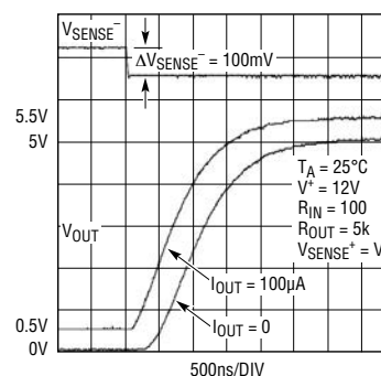
Step Response
