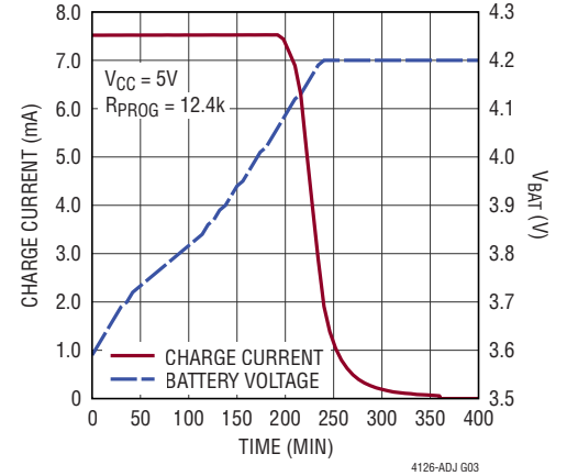
Li-Ion Battery Charge Profile
