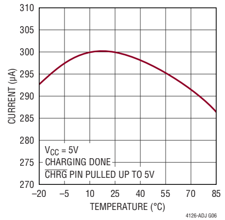
CHRG Pin Current vs Temperature
