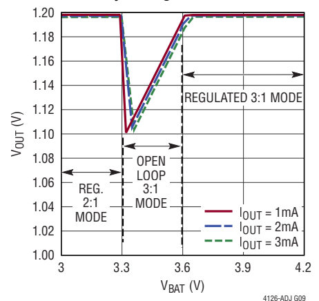
DC/DC Output Voltage vs Battery Voltage
