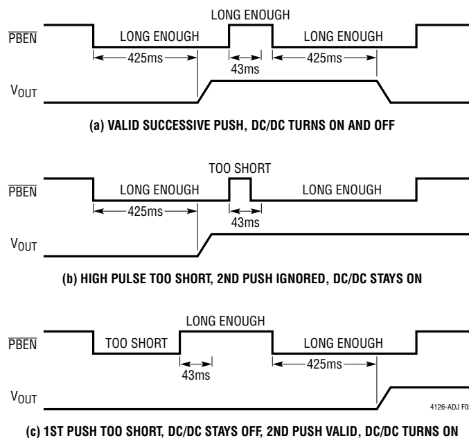
Figure 5. Various Pushbutton Scenarios
