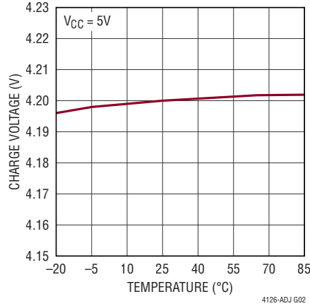
Charge Voltage vs Temperature
