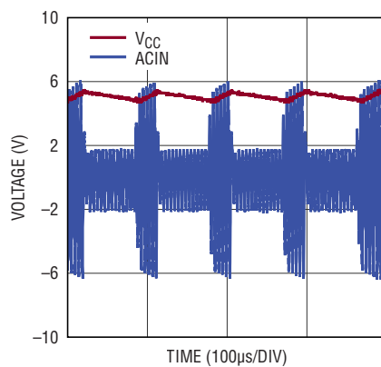
ACIN and V_{CC} Waveforms when Shunt Active
