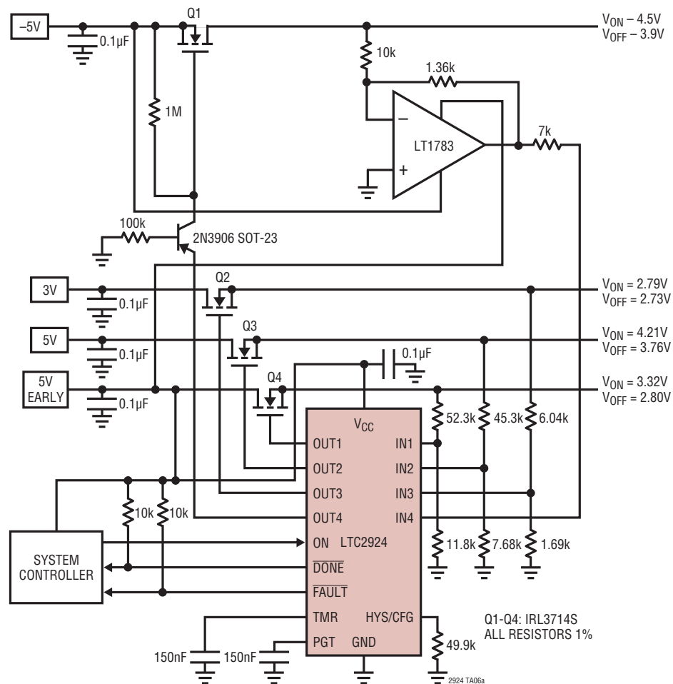
Precision Negative Rail Sequencer
