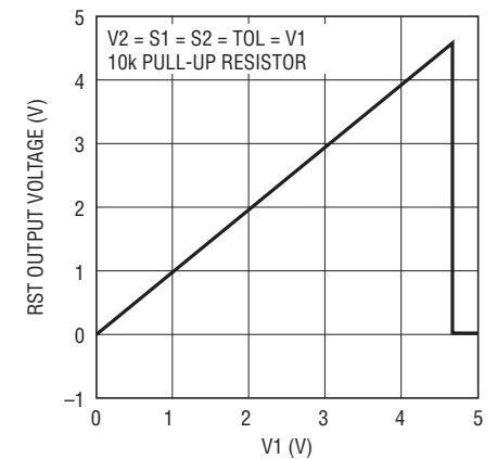
\overline{\text{RST}} Output Voltage vs V_1
