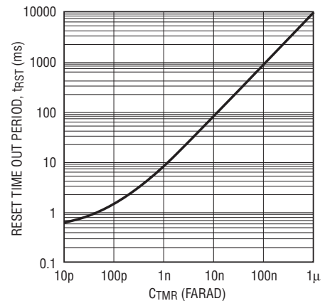
Reset Time Out Period ( t_{\text{RST}} ) vs Capacitance ( C_{\text{TMR}} )
