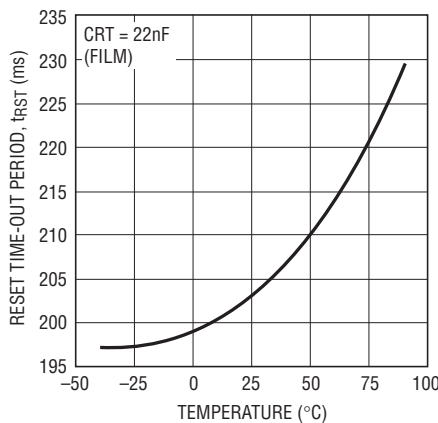
Reset Time-Out Period ( t_{\text{RST}} ) vs Temperature
