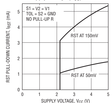
\overline{\text{RST}} Pull-Down Current ( I_{\text{RST}} ) vs Supply Voltage ( V_{\text{CC}} )
