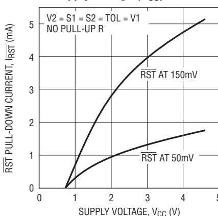
\overline{\text{RST}} Pull-Down Current ( I_{\text{RST}} ) vs Supply Voltage ( V_{\text{CC}} )
