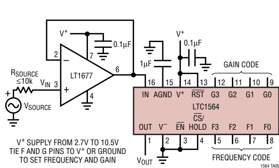
Single Supply, Very Low Noise Input Buffer for High Impedance Source Driving the Input of LTC1564
