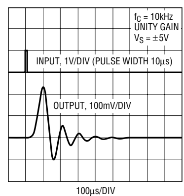
Short-Pulse Response
