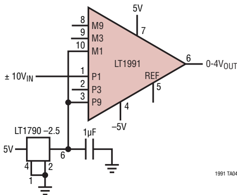
Analog Level Adaptor
