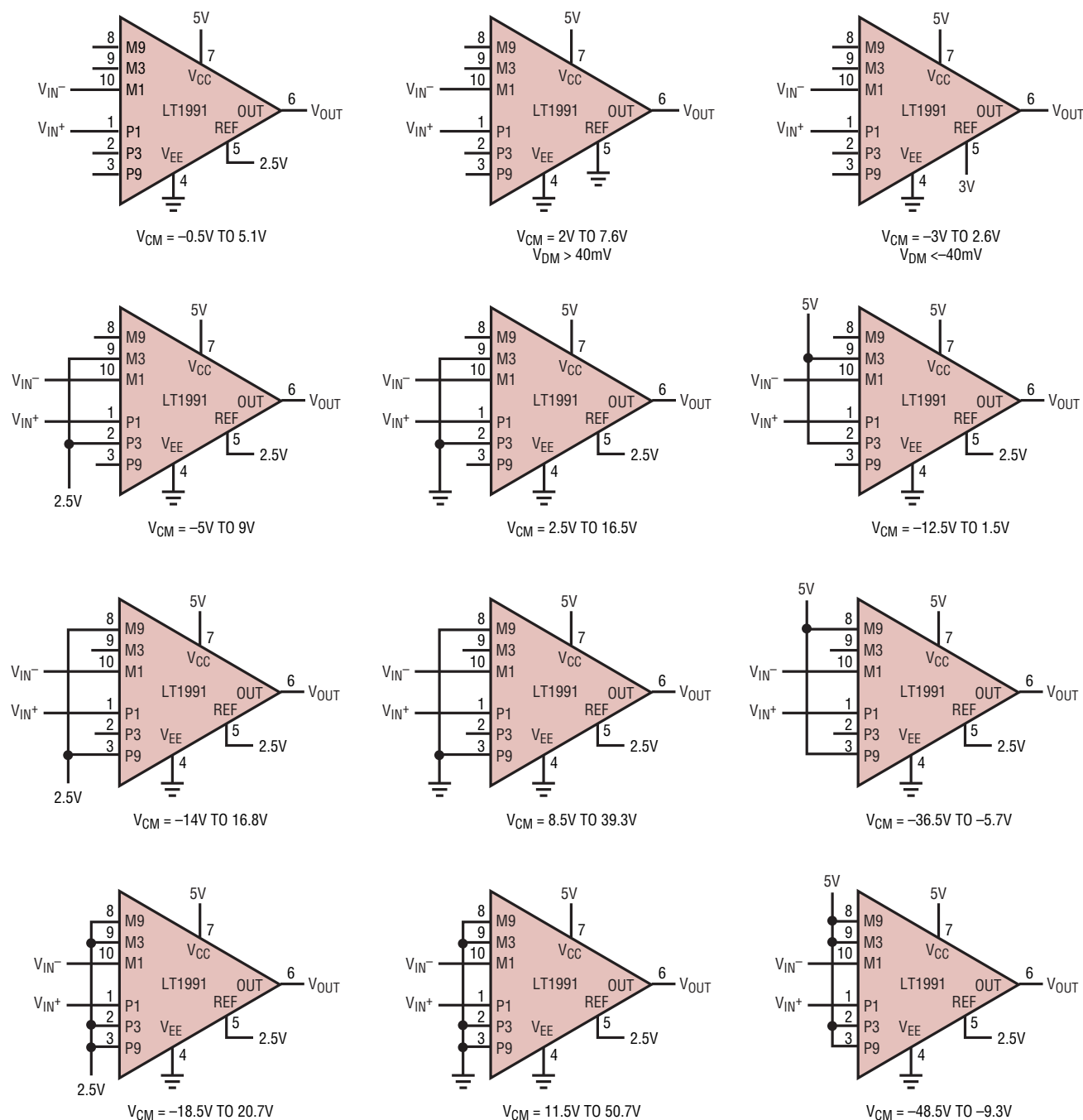
Figure 16. Common Mode Ranges for Various LT1991 Configurations on V_S = 5V , V_O = 0V ; with Gain = 1
