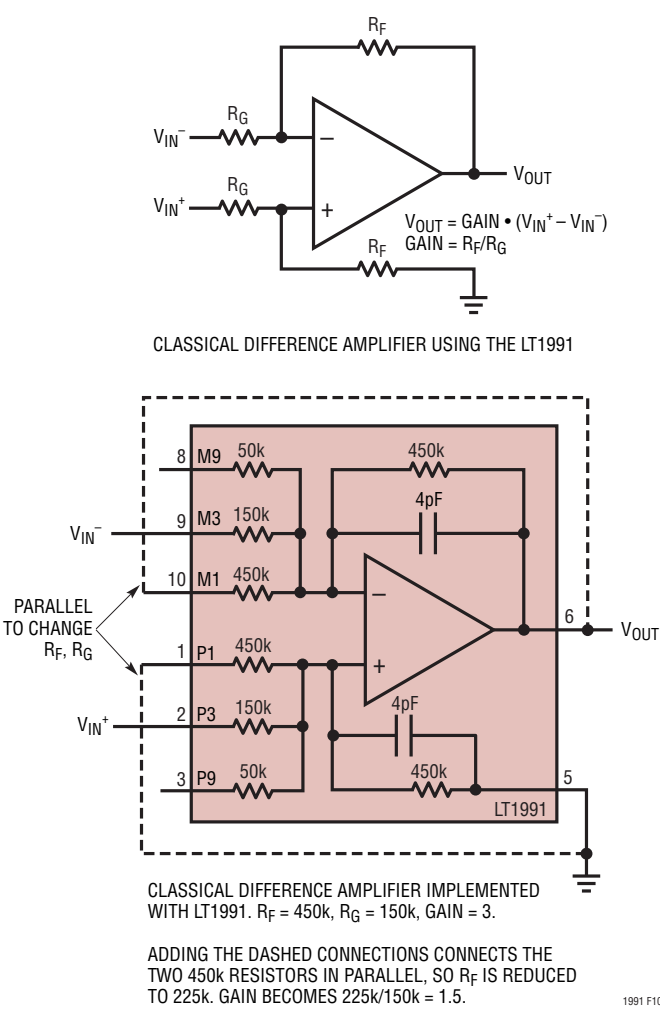
Figure 10. Difference Amplifier Using the LT1991. Gain Is Set Simply by Connecting the Correct Resistors or Combinations of Resistors. Gain of 3 Is Shown, with Dashed Lines Modifying It to Gain of 1.5. Noise Gain Is Optimal
