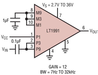
Single Supply AC Coupled Amplifier
