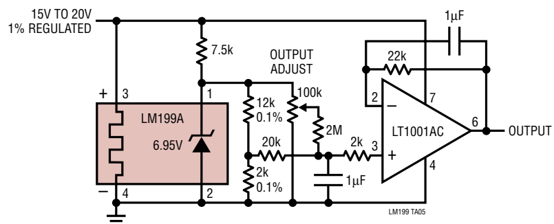
Standard Cell Replacement
