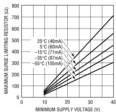
Limiting Surge Current
