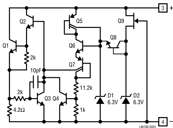
Temperature Stabilizer
