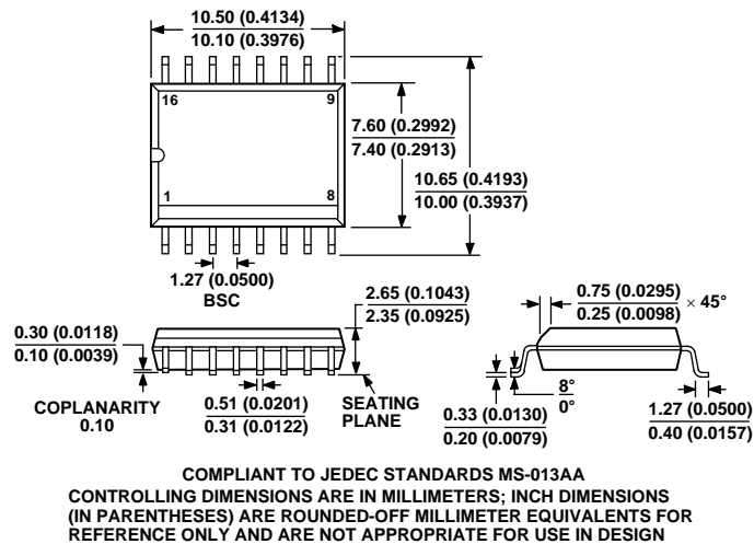
Figure 21. 16-Lead Standard Small Outline Package [SOIC]—Wide Body (RW-16)
