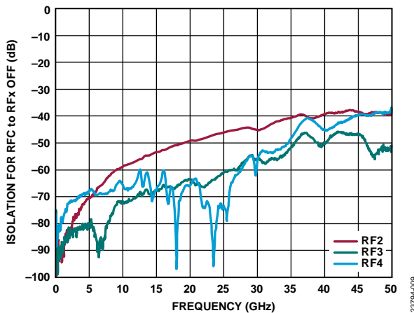
Figure 8. Isolation for RFC to RFX Off vs. Frequency, RFC to RF1 Path On
